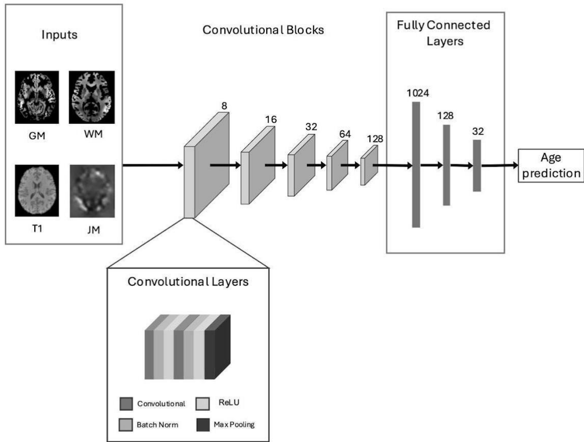
Figure 1 Overview of the CNN Model Architecture.
